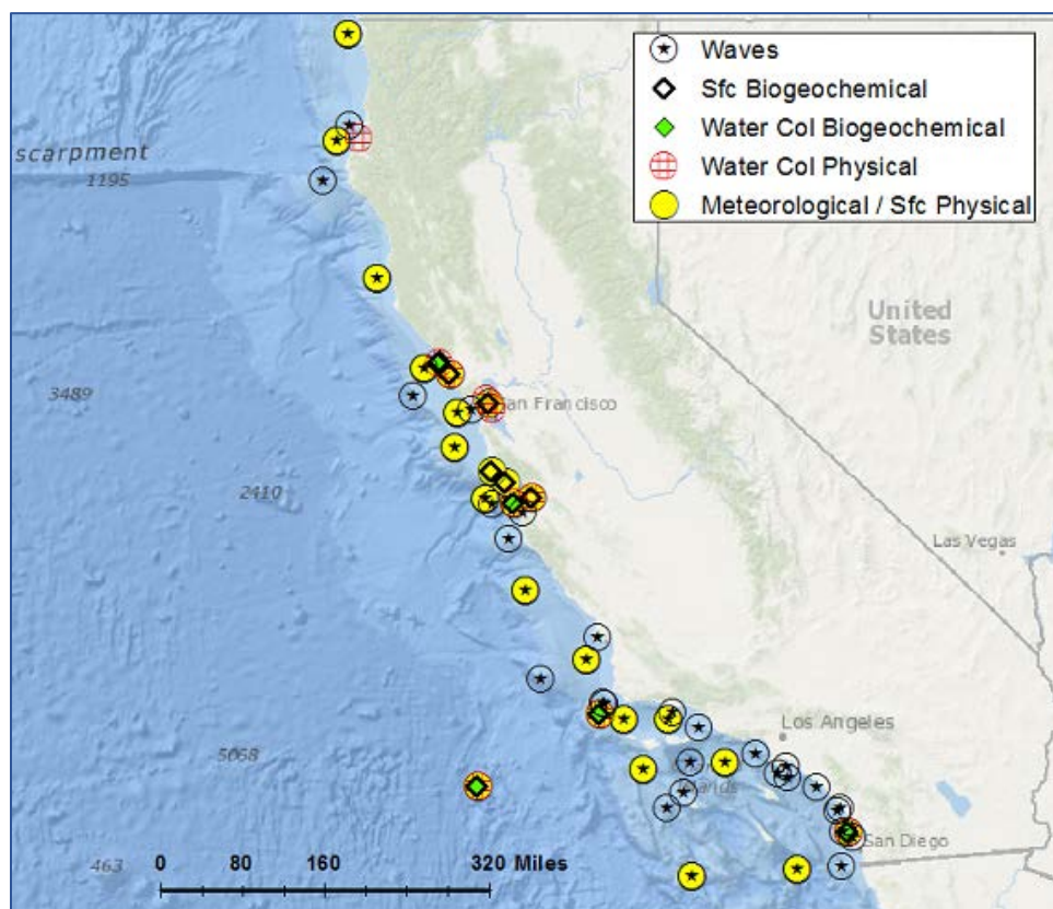
Figure 11. California: Moorings off the coast of California. NDBC operates numerous CWBs along the coast, and CDIP wave moorings are prevalent off the southern coast of California, operated with funding from the U.S. Navy, SCCOOS, and USACE. MBARI operates 4 moorings around the Monterey Bay; CO-OPS PORTS current meters are in San Francisco Bay on navigation aid buoys; and University of California San Diego Scripps Institution of Oceanography operates two moorings with water column biogeochemical observations near Pt. Conception and one near San Diego for ecosystem monitoring.
