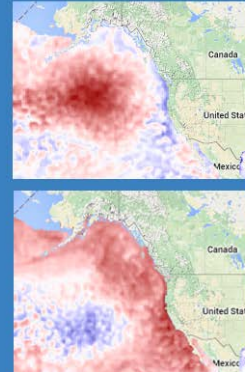
NOAA Optimal Interpolation Sea Surface Temperature Anomalies in Dec. 2013 (top) and Dec. 2014 (bottom).
