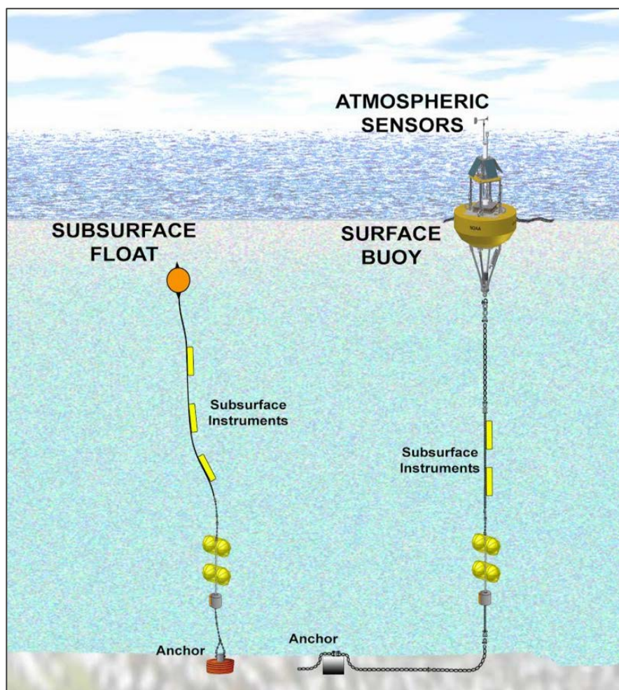
Figure 2. Coastal moorings may have a surface expression such as an instrumented data buoy or may be configured as an instrumented mooring in buoyant suspension below the surface of the ocean.
